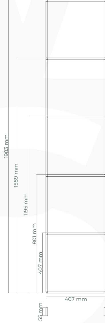
Legs Single Grid - Front
