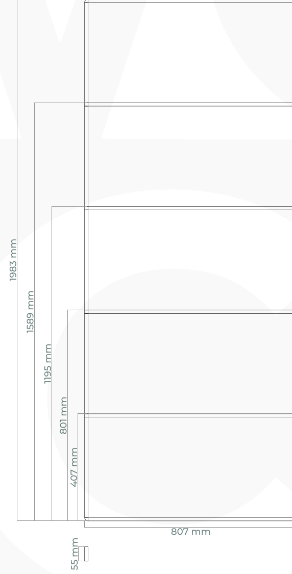
Legs Double Grid - Front
