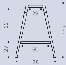
High table with wood leg Side view
