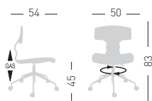
TOLO 5R Techno polymer shell, chromed base with castors. Scocca in tecnopolimero multi-colore, base in metallo cromato con ruote.
