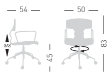
TOLO 5RB Techno polymer shell, chromed base with castors and armrests. Scocca in tecnopolimero multi-colore, base con ruote e braccioli in metallo cromato.
