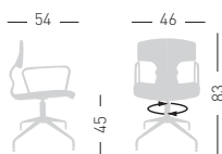
TOLO LB Techno polymer shell, chromed base and armrests. Scocca in tecnopolimero multi-colore, base e braccioli in metallo cromato.
